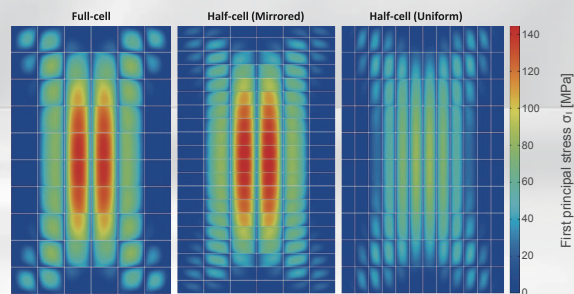
P_f = cell fracture probability First principal stress on the back side of the solar cells at 5400 Pa [1]
